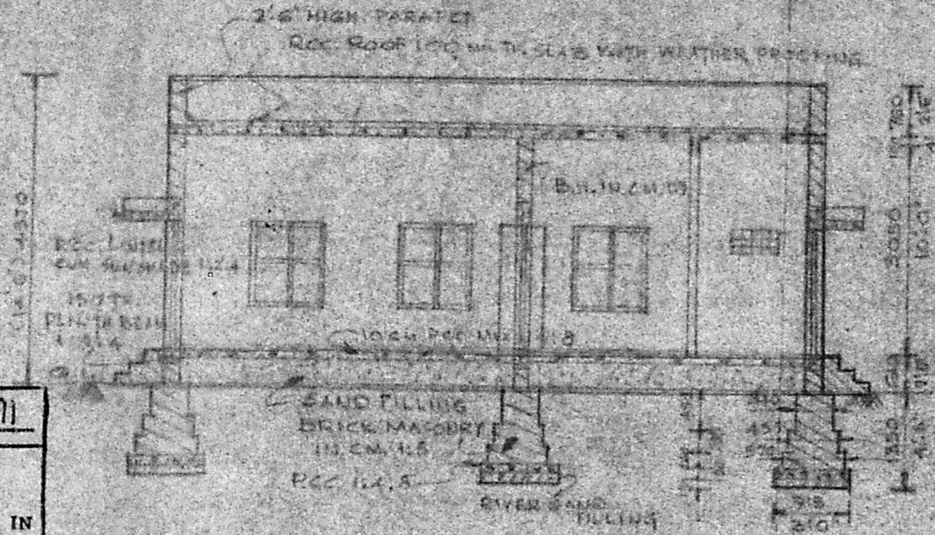
SECTION-XX
